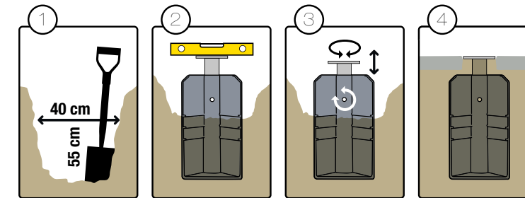
Art. nr. 6905: In-ground base XL
